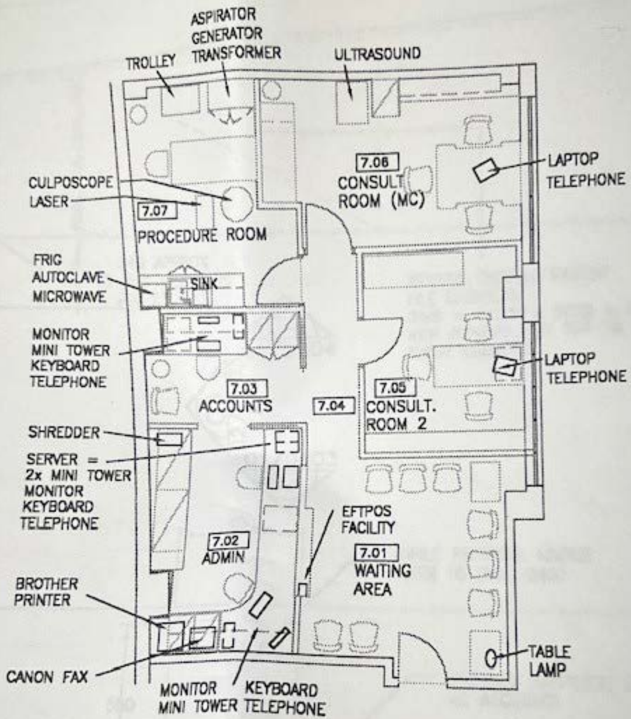
EQUIPMENT LAYOUT PLAN - 1:100
